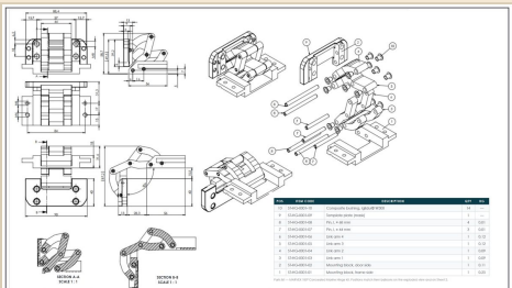
FIG. 03 — GENERAL ARRANGEMENT & PARTS LIST · SHEET 1 OF 2 · NOT TO SCALE
